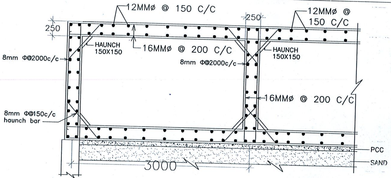
SECTIONAL ELEVATION-XX
